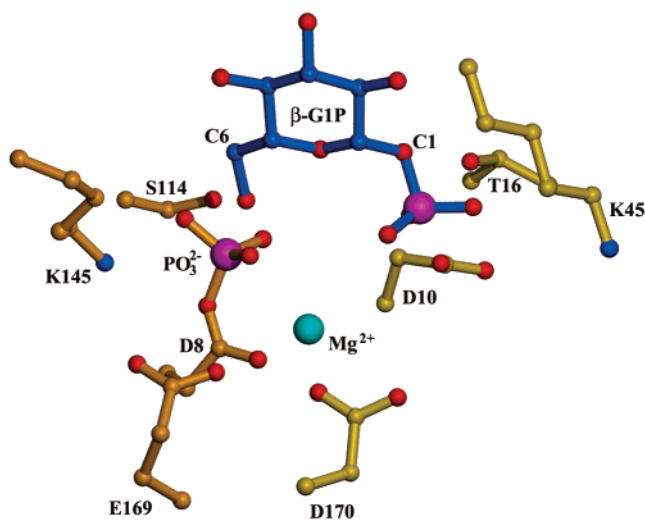
FIGURE 4: The active site of \beta -PGM showing the docked substrate glucose-1 phosphate and polar residues within 6 Å to the sugar C(1) and C(6). The residues located proximal to C(6) of the sugar are shown in gold and those located proximal to C(1) of the sugar are shown in yellow.
