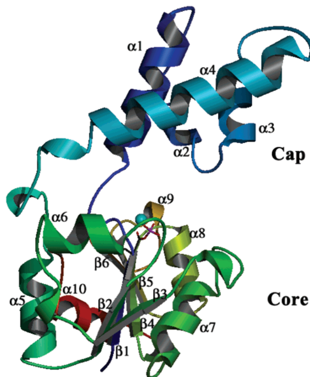
FIGURE 1: Structure of \beta -phosphoglucosyltransferase. A schematic representation with the strands and helices labeled sequentially with color ramped from blue to red from N- to C-terminus. The aspartyl phosphate group (Asp8) is shown as a stick model and Mg 2+ ion as a cyan sphere.
